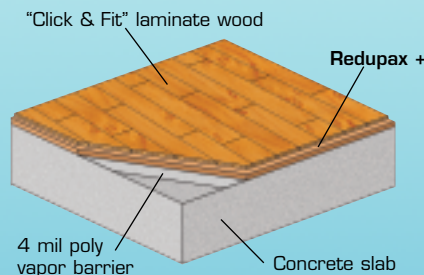
Typical Concrete Slab Construction
